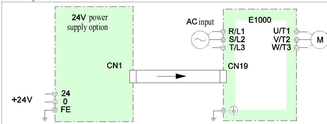
Connection Diagram
