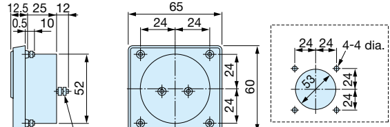
Dimensions (mm)
