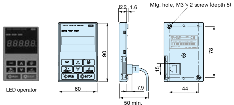
Dimensions (mm)
