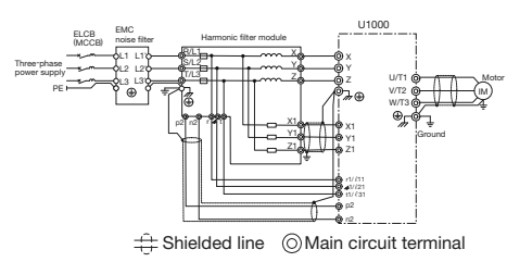
Wiring Diagram c
